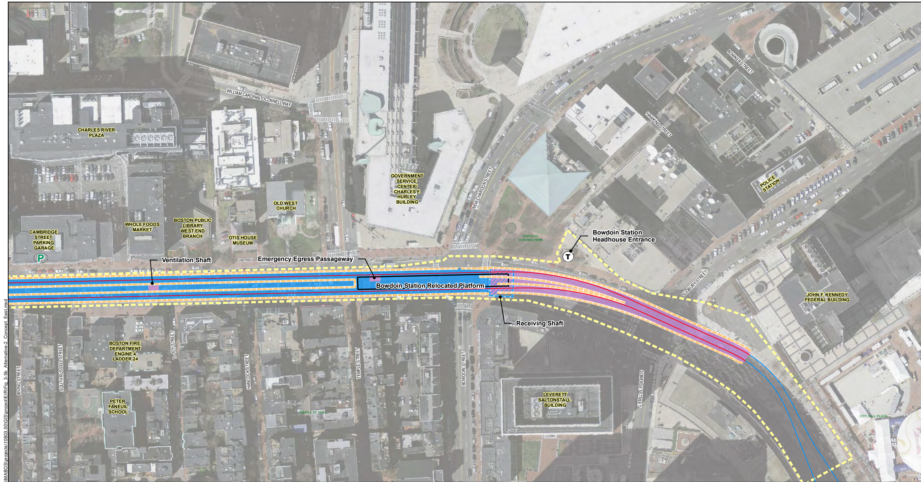
Figure 3-5b Alternative 2: Bowdoin Station Relocated Conceptual Layout (East)
