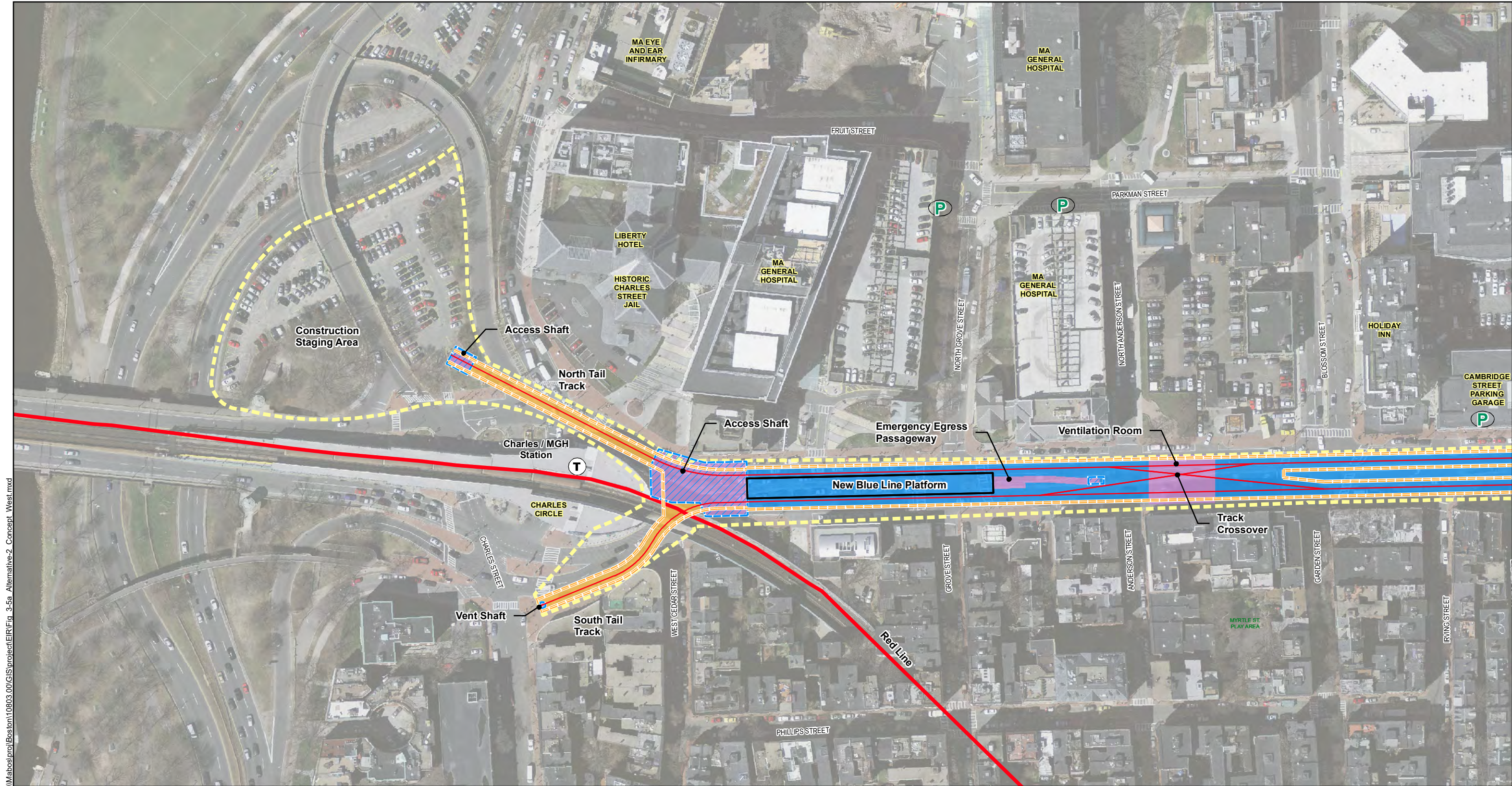
Figure 3-5a Alternative 2: Bowdoin Station Relocated Conceptual Layout (West)
