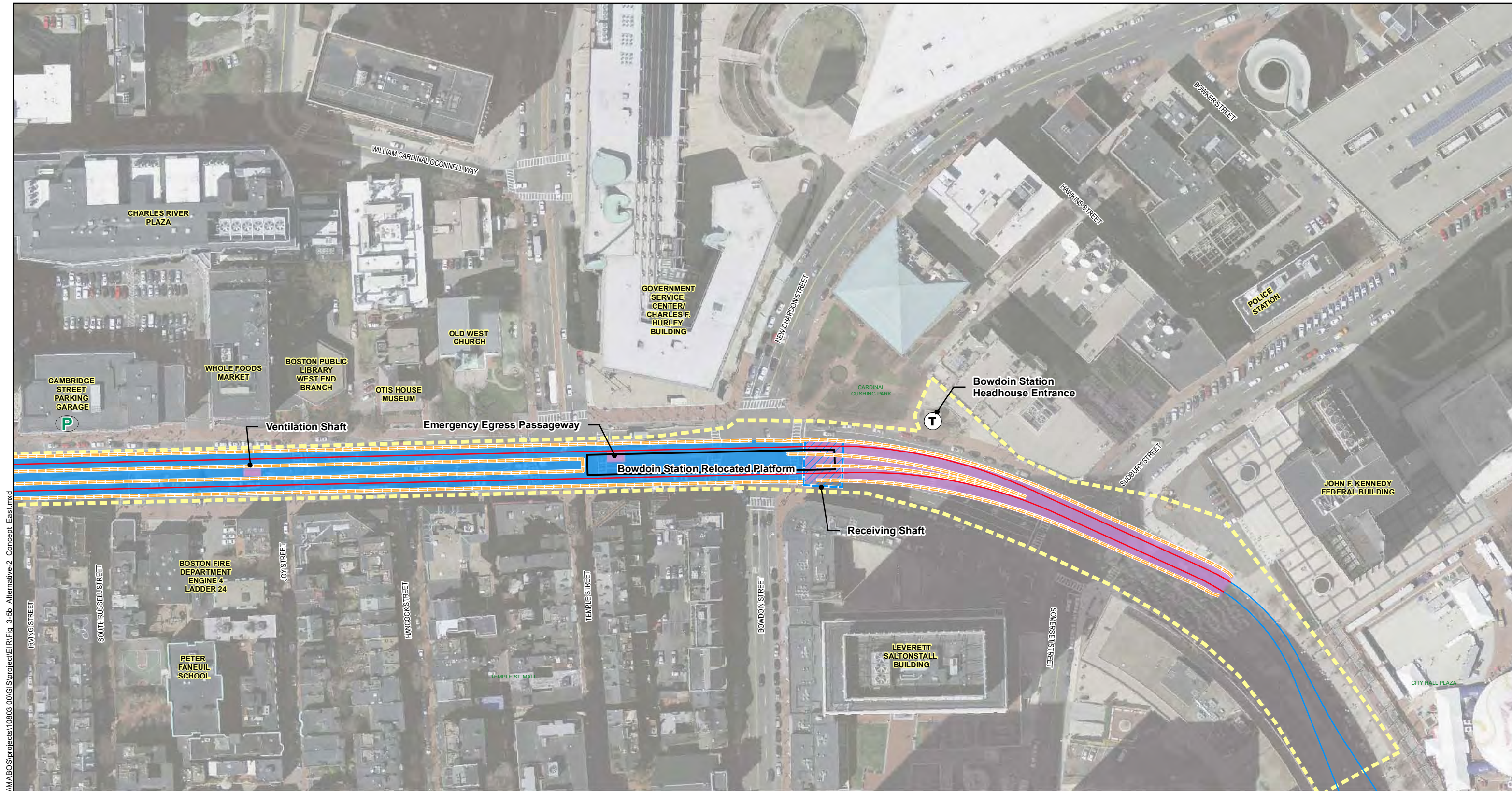
Figure ES-4b Alternative 2: Bowdoin Station Relocated Conceptual Layout (East)
