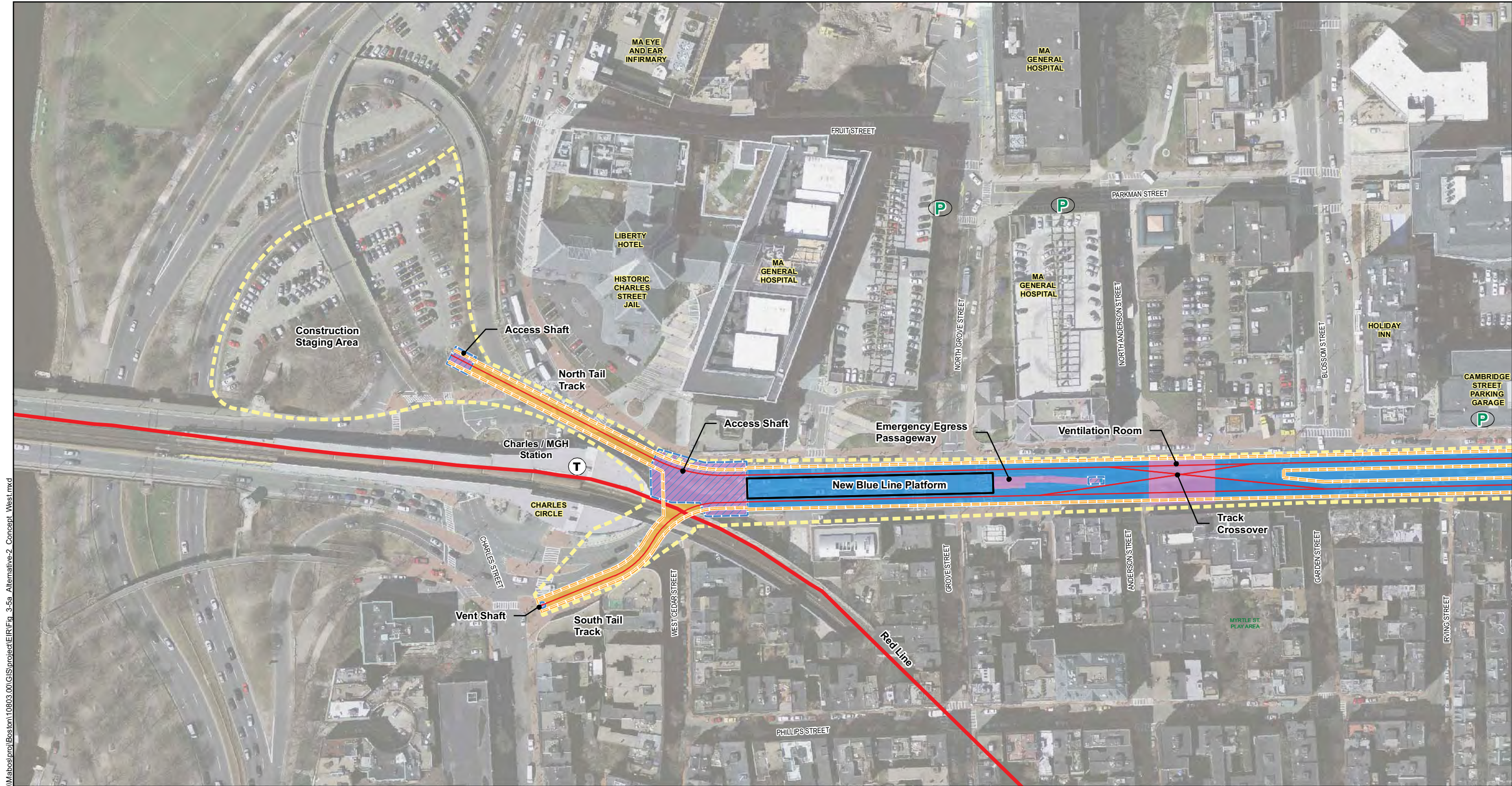
Figure ES-4a Alternative 2: Bowdoin Station Relocated Conceptual Layout (West)
