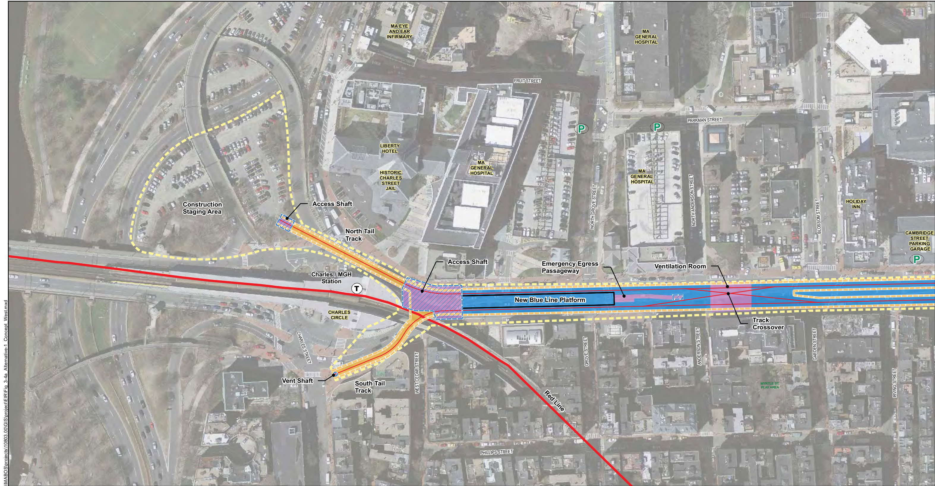
Figure ES-2a Alternative 1: Bowdoin Station Eliminated Conceptual Layout (West)
