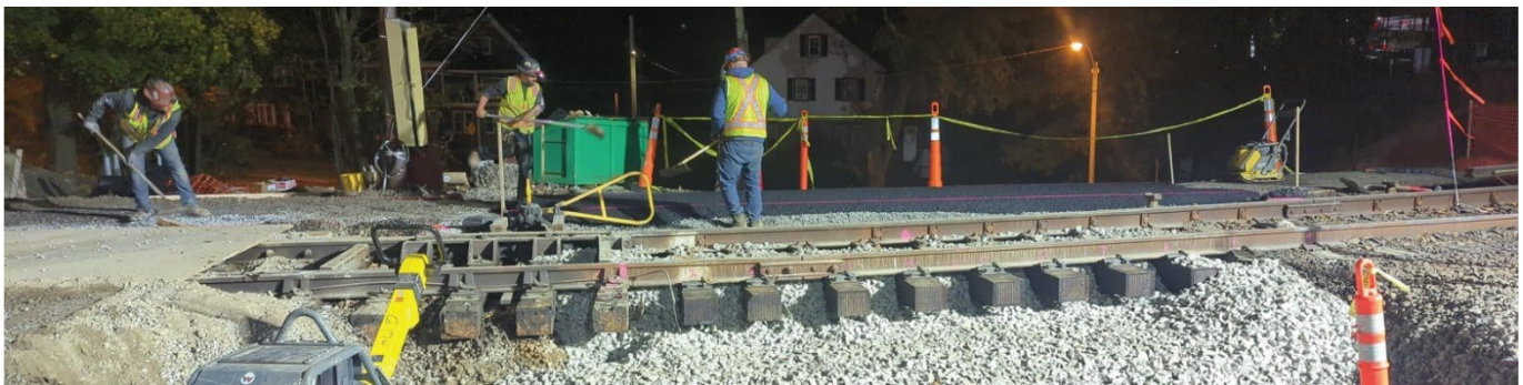
Crews install power conduit under Codman Yard tracks
