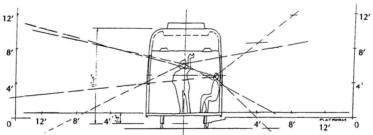
Fig. 2-100 Green Line Vehicle-Platform Sightlines
