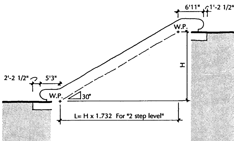
Fig. 2-52 Escalator Dimensions
