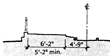
Fig. 2-12 Platform Width at Surface Station
