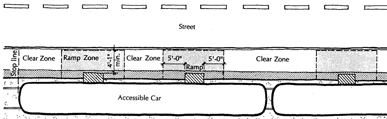
Fig. 2-13 Critical Dimensions at Surface Stations
