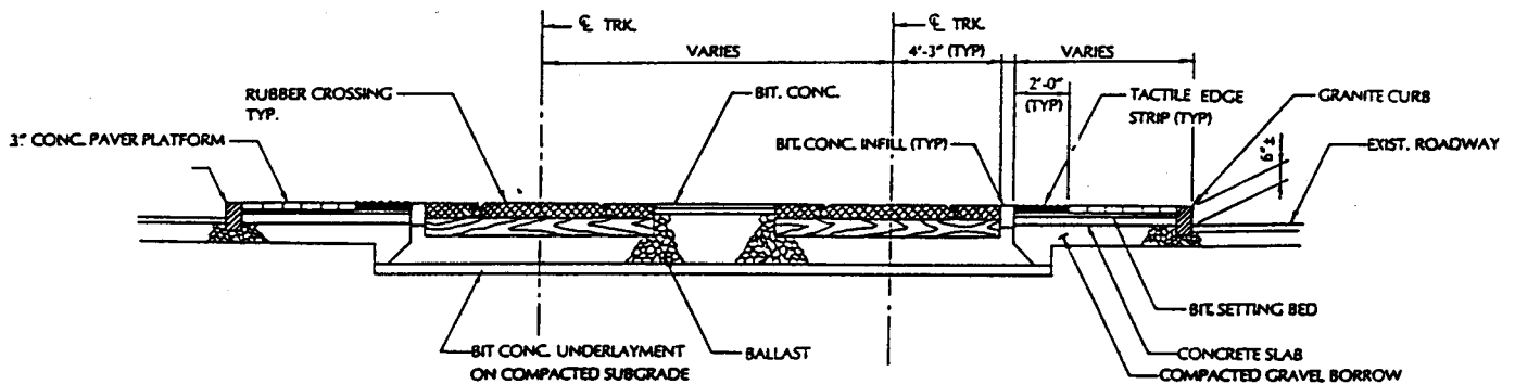
Fig. 2-74 Rubber Grade Section at Platform Area (B)
