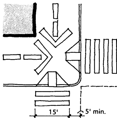
Fig. 2-22 Corner Curb Ramps
