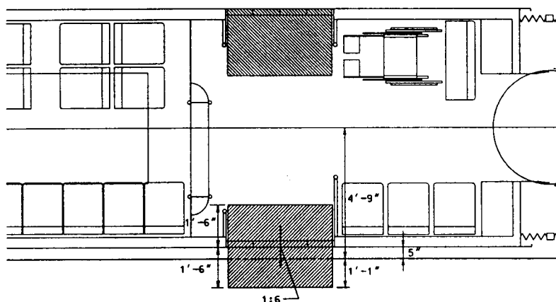
Fig. 3-2 LFV Ramp (Plan View)
