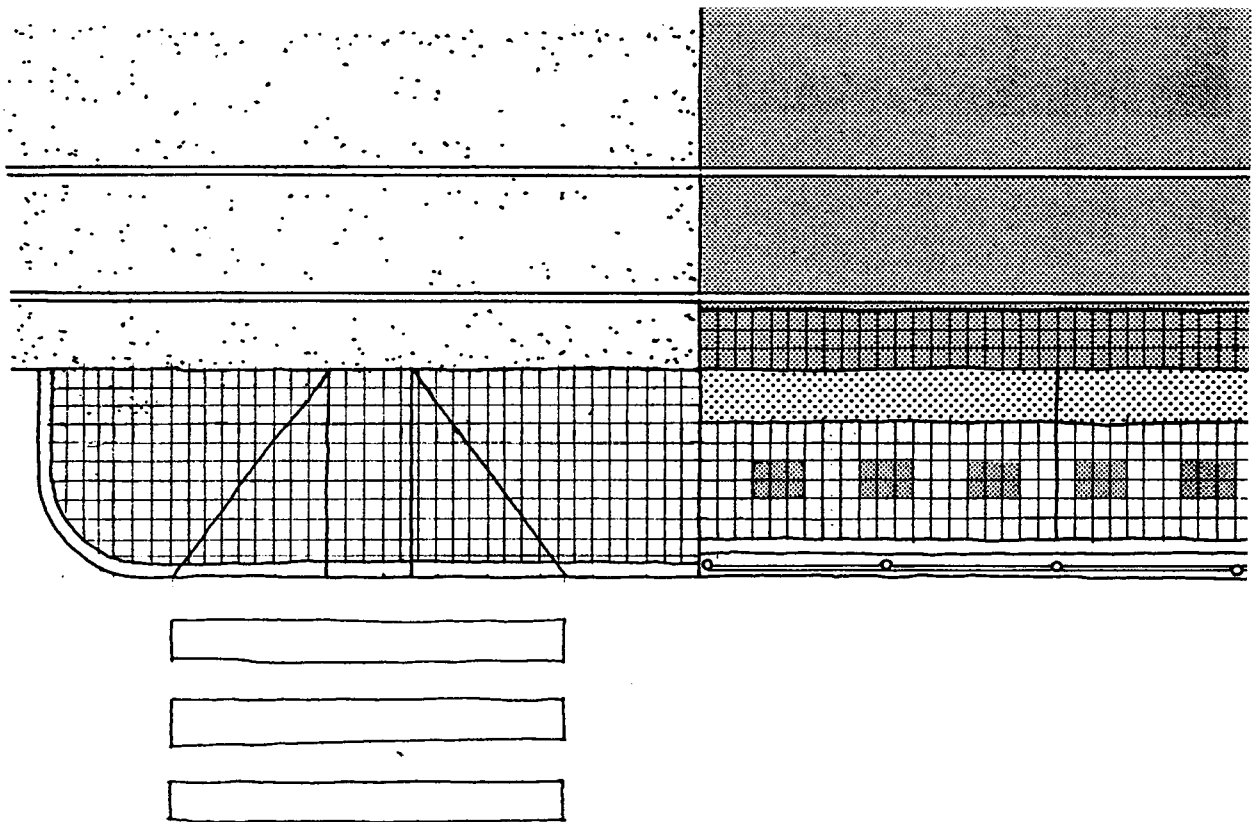
Fig. 2-87 Possible Paving Pattern at Narrow Platform, Alternative #2
