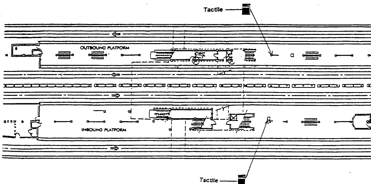
Fig. 2-99 Prototypical Subway Station Signage Layout - Kenmore Station - Platform Level
