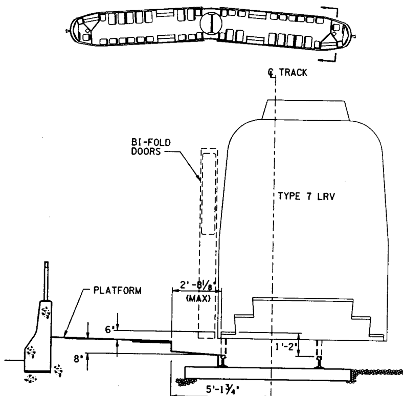
Fig. 3-12 Type 7 LRV at Raised Platform on Inside of Curve (R=180')
