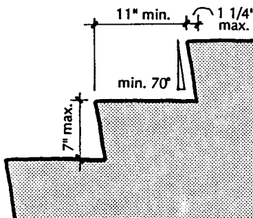
Fig. 2-54 Riser/Tread Detail
