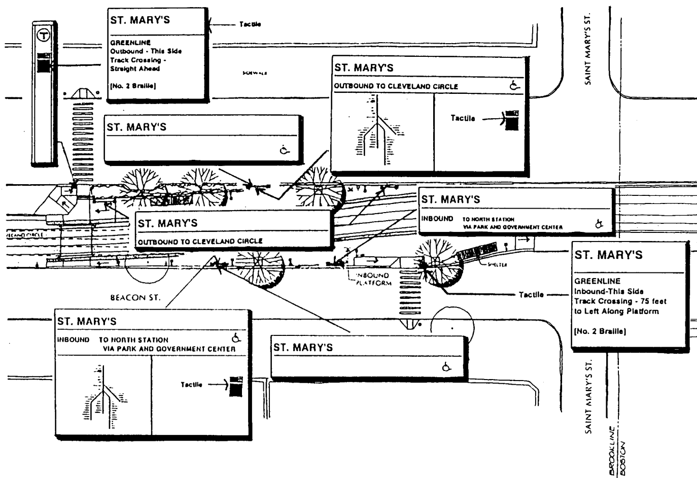
Fig. 2-96 Prototypical Surface Station Signage Layout - St. Mary's Street
