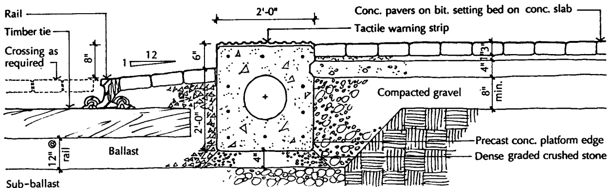
Fig. 2-83 Detail at Surface Station Platform
