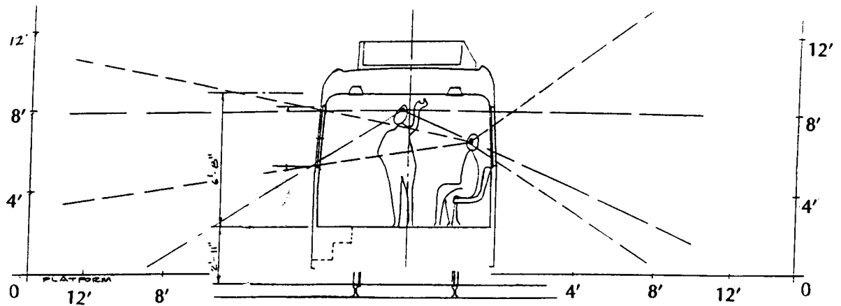
No. 7 Car - Sightlines
