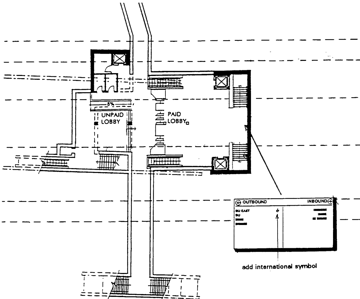
Fig. 2-98 Prototypical Subway Station Signage Layout - Kenmore Station - Mezzanine Level
