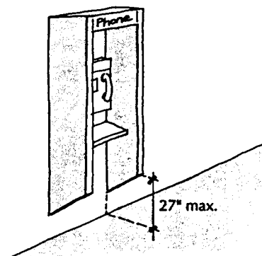
Fig. 2-21 Mounted Objects Along Accessible Route
