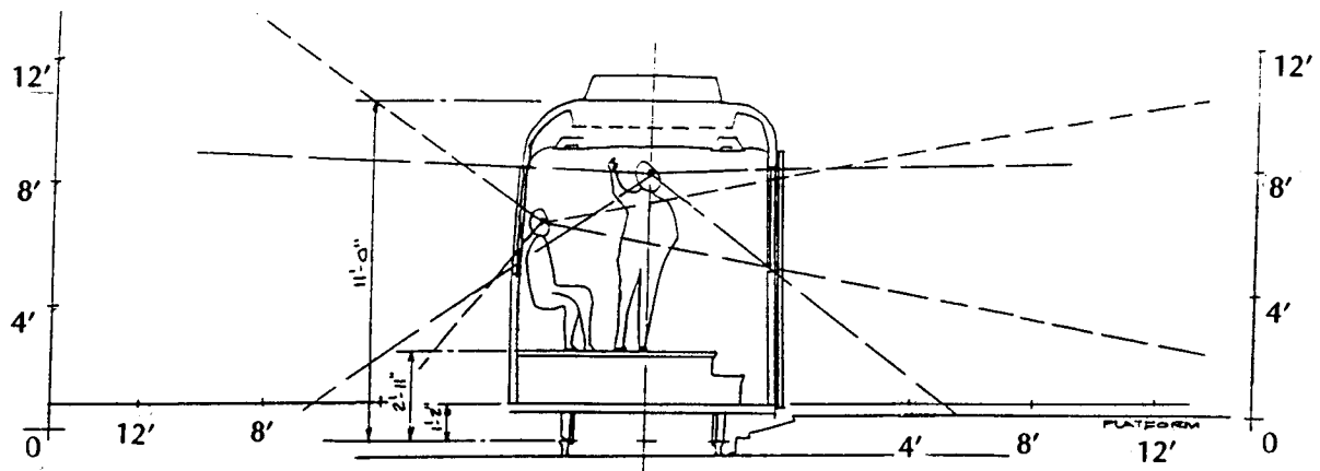
LFV - Upper Floor Sightlines
