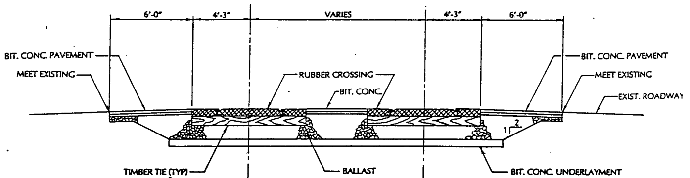
Fig. 2-73 Rubber Grade Crossing Section at Intersection (A)
