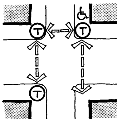
Fig. 2-4 Accessible Route to Subway Entrance
