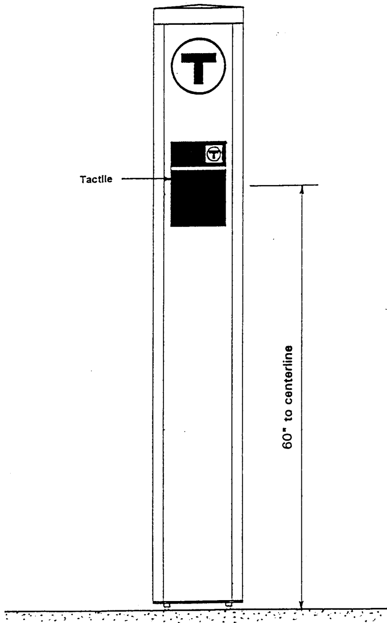
Fig. 2-92 Tactile Entrance Signs at Curb Ramp
