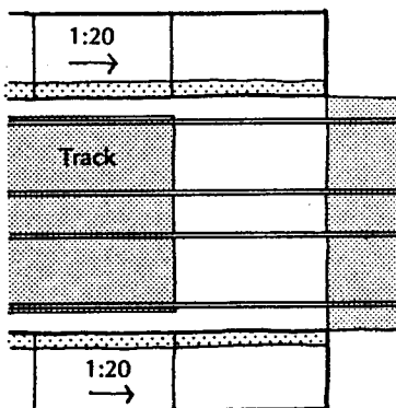
Fig. 2-40 Accessible End of Track Crossing
