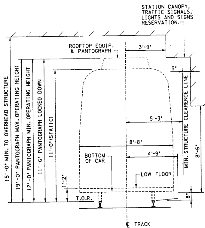
Fig. 3-6 LFV Clearances
